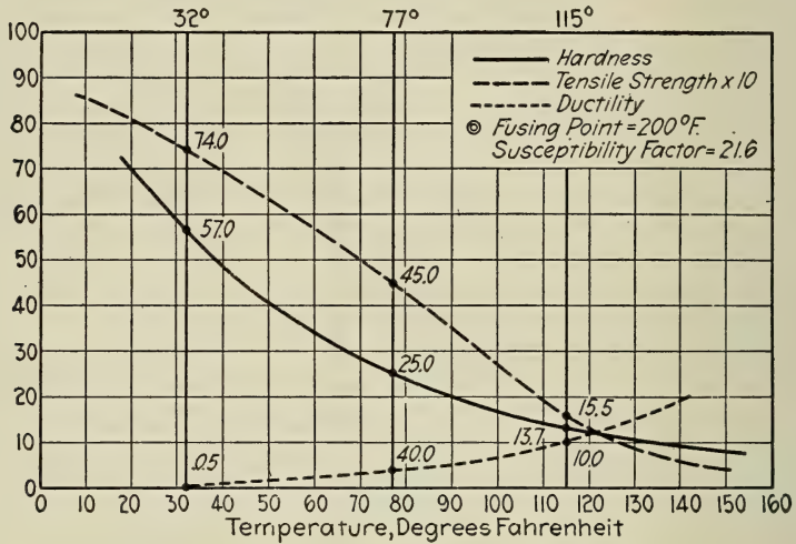
FIG. 54.—Chart of Physical Characteristics of Fluxed Trinidad Grahamite Mixture.
